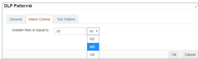
Figure 8: Match Criteria tab for a File Size data pattern.
